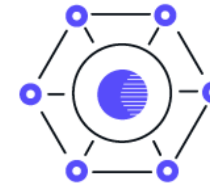
ORGANISMS
